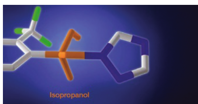
Revysol's triazole 'head' sits on the 'neck' of a slim isopropanol unit.
